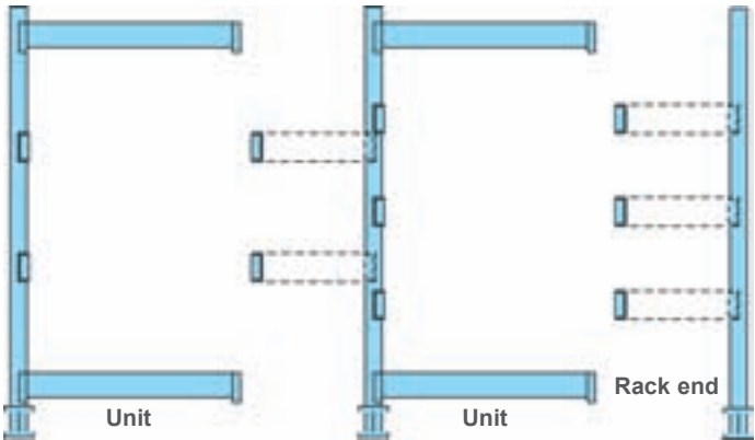
Each unit supplied with right-hand reel holders (as specified) that fasten to next unit or rack end.
